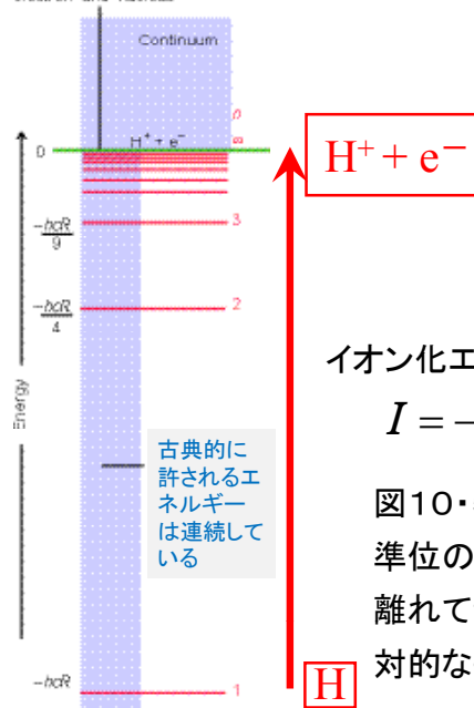
Energy of widely separated stationary electron and nucleus
